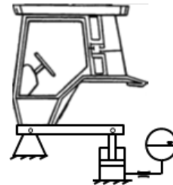
Cab suspension
