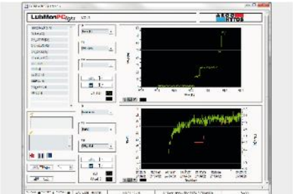
Software
